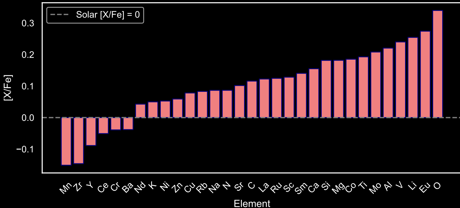
Abundance Pattern for GALAH Red Giants: Star Field [105] (N=61)
