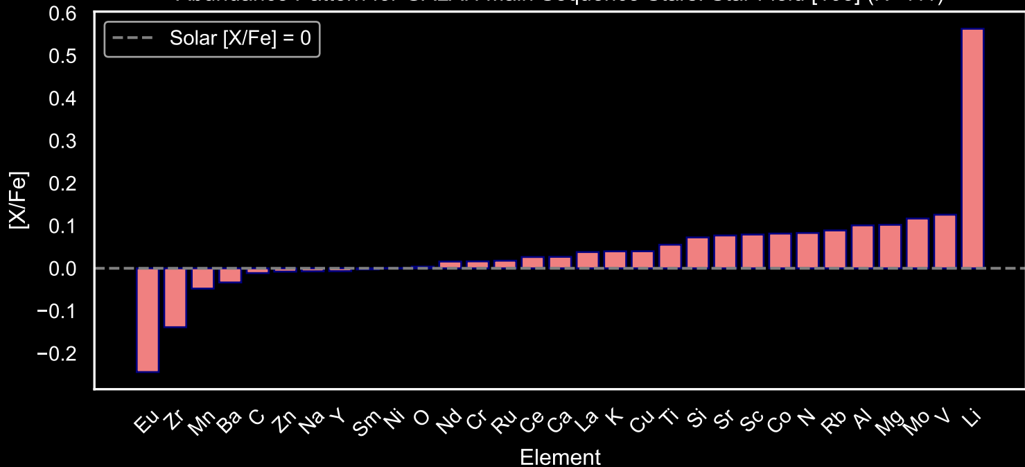
Abundance Pattern for GALAH Main Sequence Stars: Star Field [105] (N=111)
