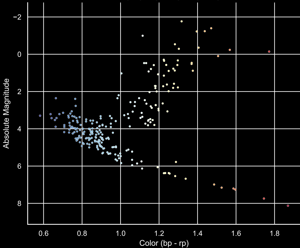
GALAH Hertzprung-Russel Diagram Field [105] Ra [322.58] Dec [-16.73]
