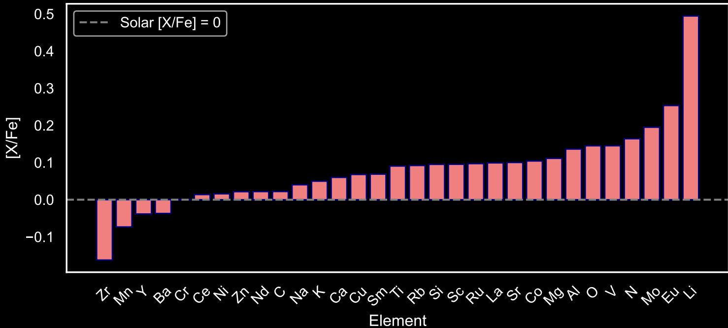
Abundance Pattern for GALAH Star Field [105] (N=243)
