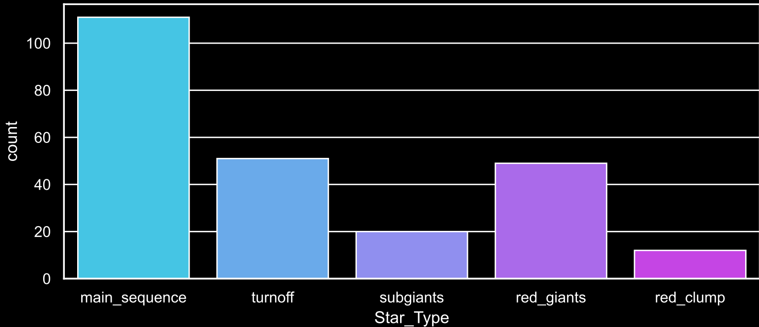
Field [105] Count plot of Star Type
